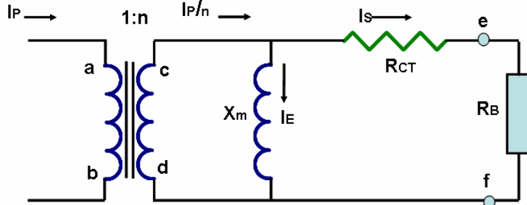
Figure 1a. Simplified equivalent circuit of a current transformer
