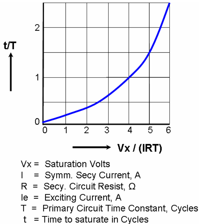
Figure 8. Time to saturate as a function of the saturation voltage and secondary circuit resistance
